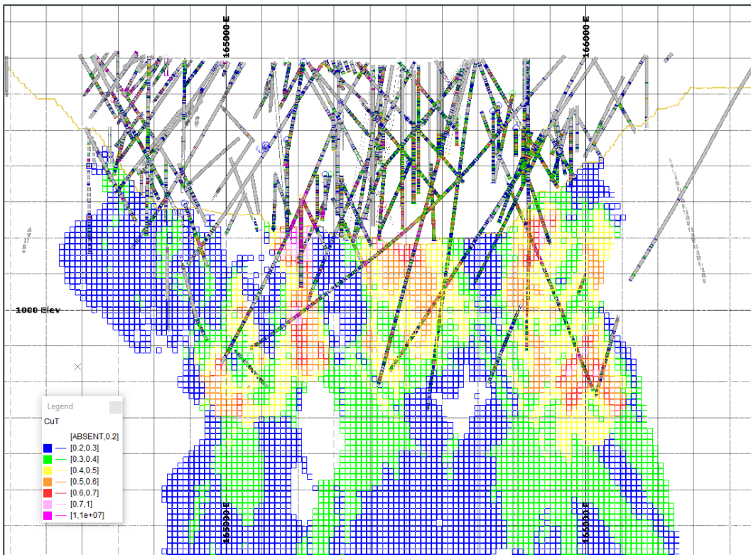
Figure 7: Swath Plots for Mo (%), TCu (%) and Au (g/t): in three orthogonal directions
