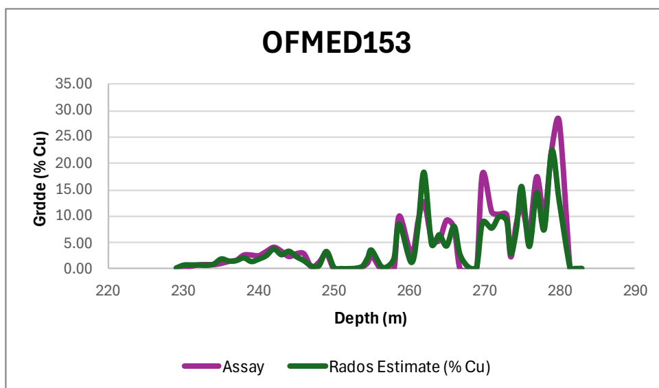
Figure 4: RADOS™ XRF scan readings versus ICP assay results for OFMED151, OFMED152 and OFMED153.
